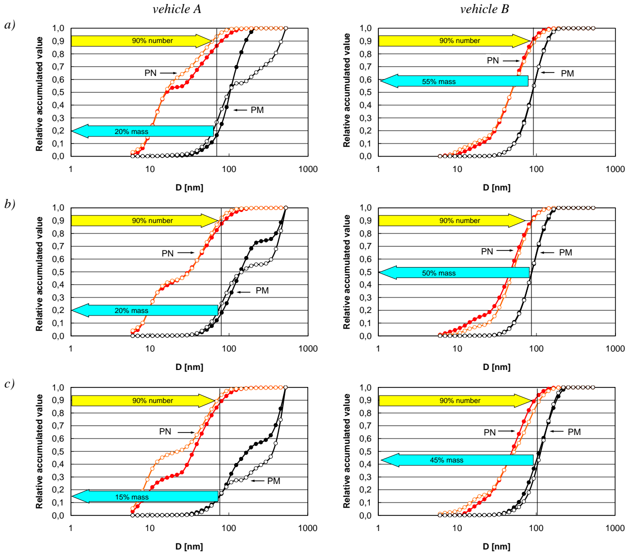
Fig. 11. Relative accumulated value of the particle number (PN) and mass (PM) as a function of its size recorded on different road portions for tested vehicles A and B: a) urban, b) extra urban, c) expressway; ● – drive with load, ○ – drive without load
