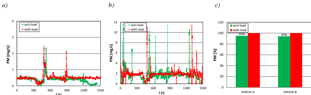
Fig. 6. PM emission rate on the expressway road portion: a) vehicle A, b) vehicle B, c) relative values
