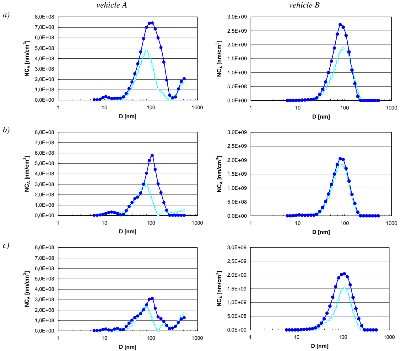
Fig. 9. Normalized surface concentration NC_A of PM as a function of diameter D recorded on different road portions for the tested vehicles A and B: a) urban, b) extra urban, c) expressway; ● – drive with load, ○ – drive without load
