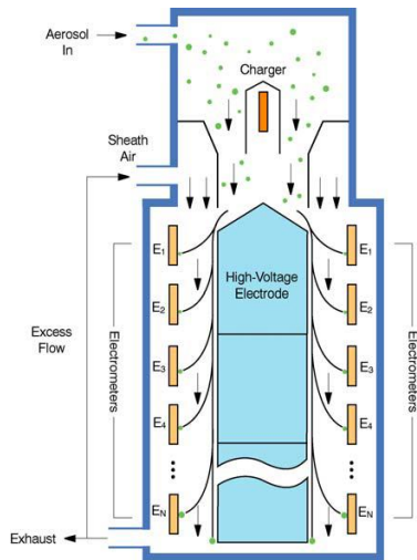
Fig. 2. Schematics of the EEPS 3090 particle sizer
