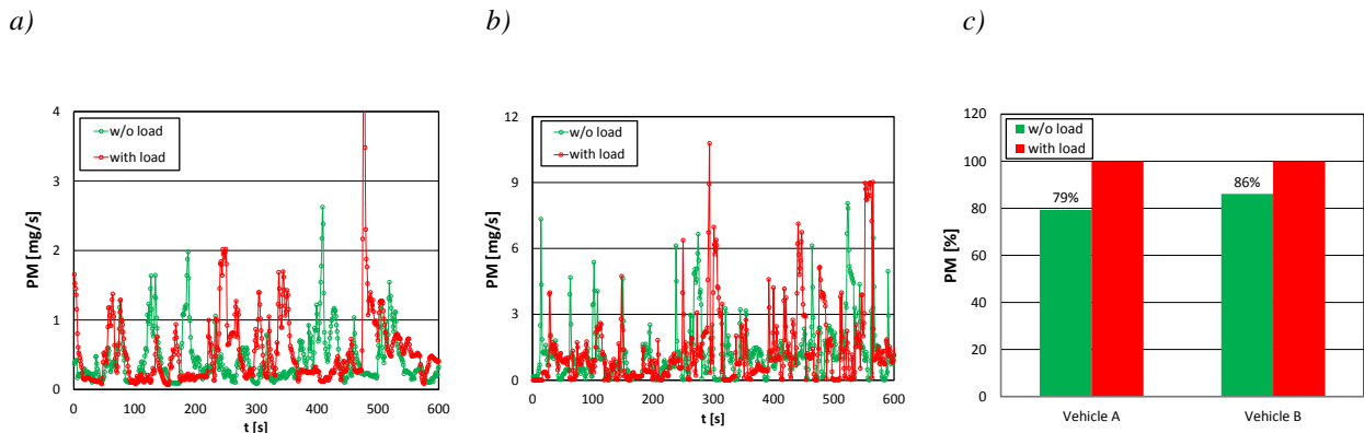
Fig. 4. PM emission rate on the urban road portion: a) vehicle A, b) vehicle B, c) relative values
